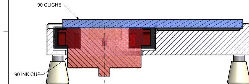
SECTION A-A SCALE 3 / 4
