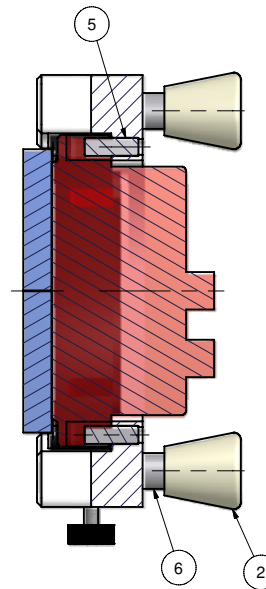
SECTION C-C SCALE 3 / 4
